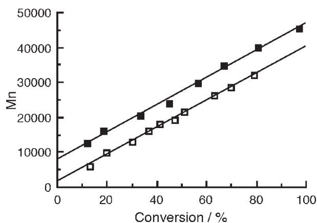
Figure 1. Dependence of PMMA molecular weight M_n on monomer conversion with catalysts 3a (■) and 3b (□). See Table 1 for reaction conditions.
