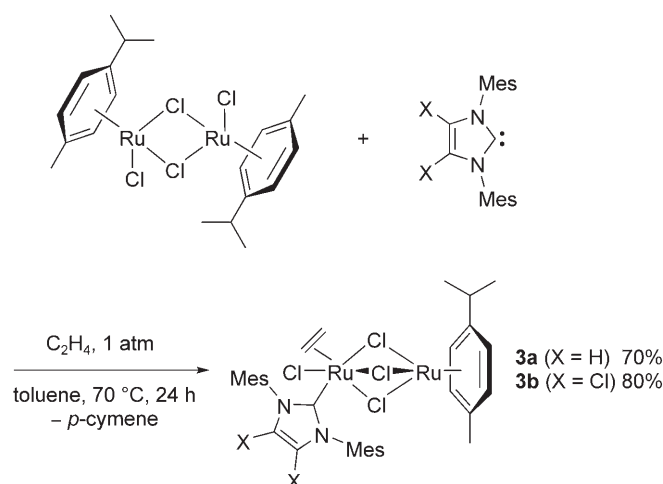
Scheme 1. Synthesis of homobimetallic ruthenium-NHC complexes 3a and 3b .
