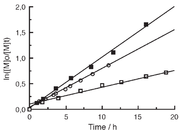
Figure 2. Time dependence of \ln([M]_0/[M]_t) for the ATRP of MMA at 85°C with catalysts 2a (○), 3a (■), and 3b (□). See Table 1 for reaction conditions.
