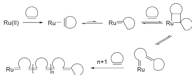
Scheme 2. Possible mechanism for the ROMP of cycloolefins.
