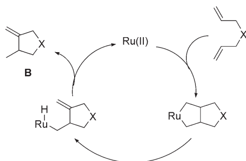
Scheme 3. Catalytic cycle for the cycloisomerization of \alpha,\omega -dienes.
