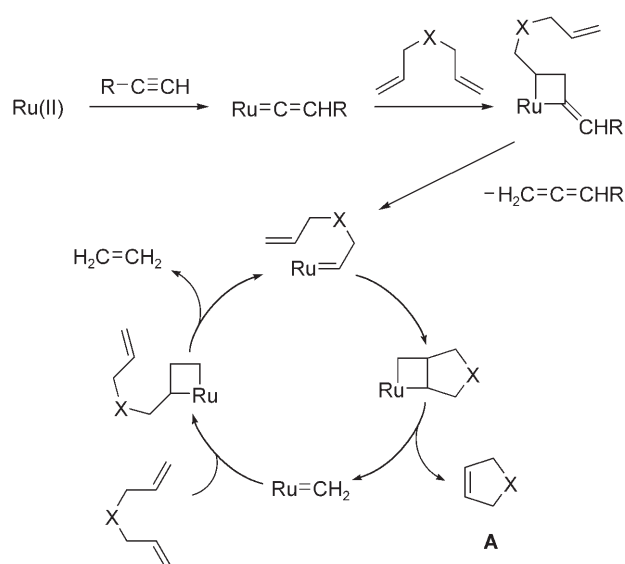
Scheme 4. Catalytic cycle for the RCM of \alpha,\omega -dienes in the presence of a terminal alkyne.
